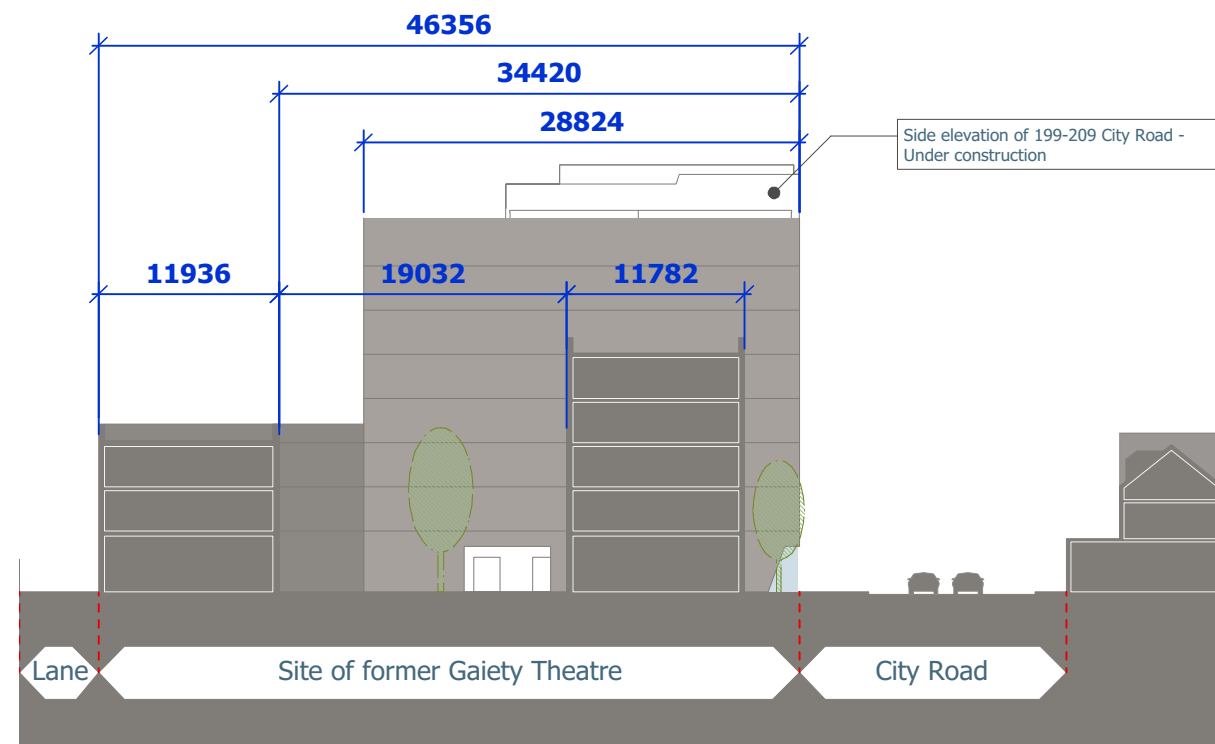
Illustrative - Section
