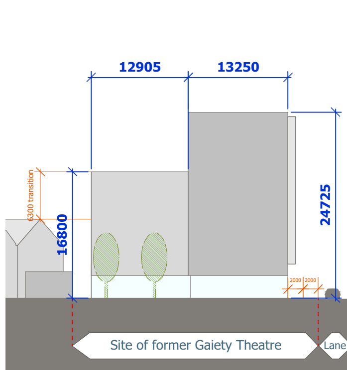
Illustrative - Elevation
