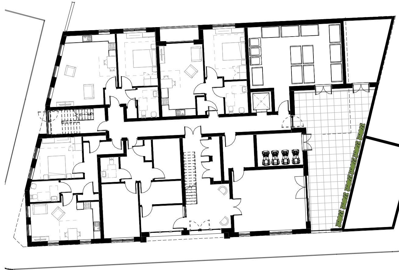
01 PROPOSED GROUND FLOOR PLAN 1 : 100
