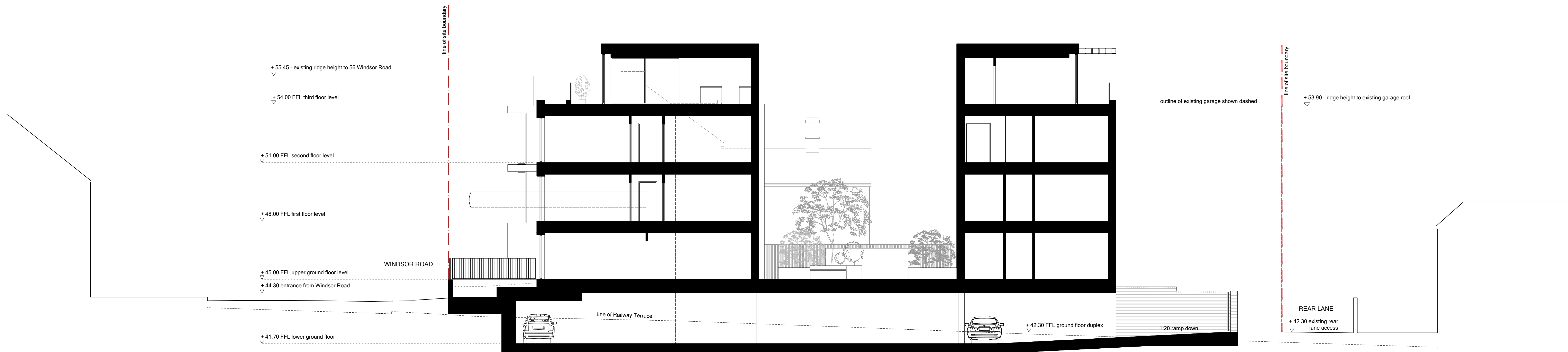
PROPOSED SECTION A-A 1:100
